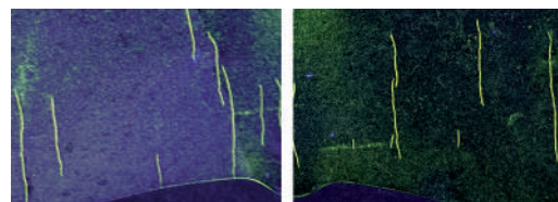
The integrated special filter ensures better crack detection (right) by avoiding disturbing reflections (left)
